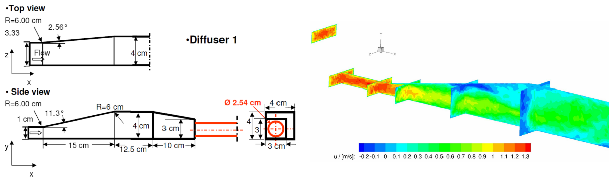
Figure 1: Geometry of the diffuser considered (Cherry et al., 2008) (left) and the instantaneous velocity field obtained by LES (right).
